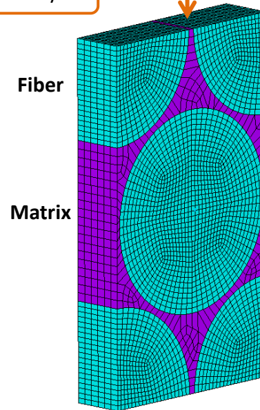
RVE, hexagonal array
